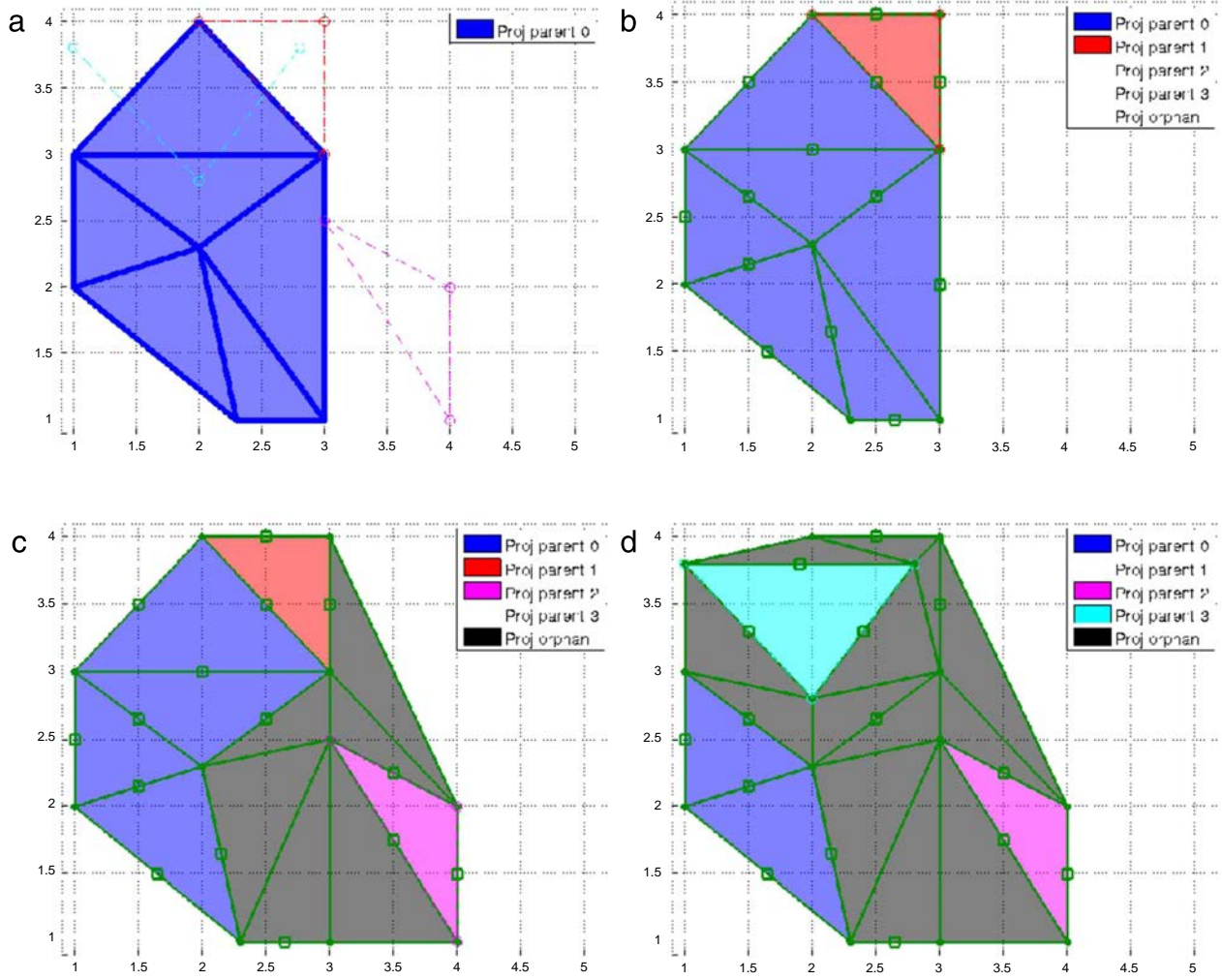
Fig. 8. The projection parent status of each triangle (same example as in Fig. 7): (a) candidate triangles and initial mesh M ; (b) first insertion, mesh M^* ; (c) second insertion, mesh M^{**} ; (d) third insertion, mesh M^{***} .
