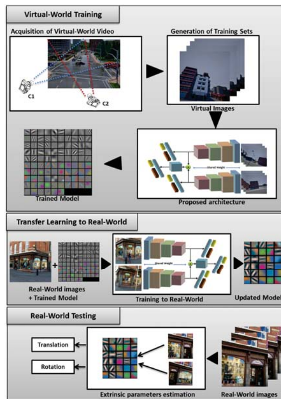
Figure 2: Training and testing processes.
