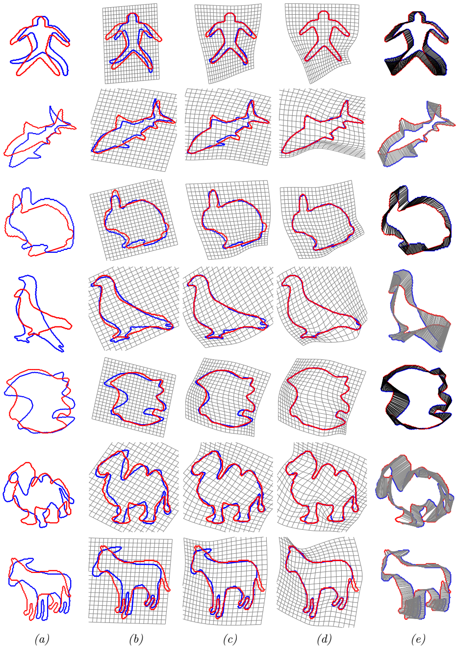
Fig. 3. Registration results of 2D shapes ([19], [20]) using the proposed approach (SD-FFD): (a) initial configurations of data sets (blue) and model sets (red); (b) results with \lambda = 10^5 ; (c) results with \lambda = 10^2 ; (d) results with \lambda = 1 ; (e) the obtained FFD control lattice results in a very dense correspondence over the whole region.
