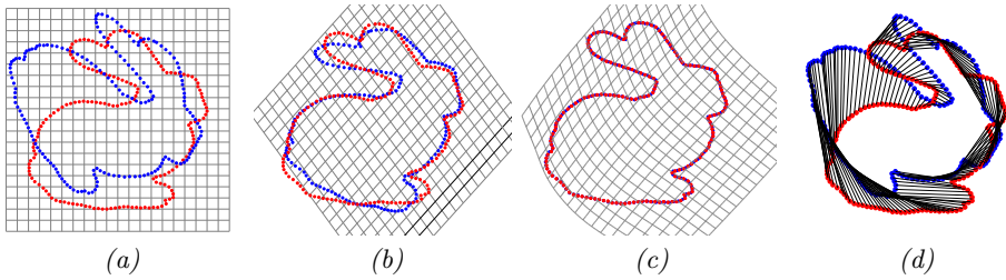
Fig. 1. The proposed method (SD-FFD): (a) initial configuration of the data set (blue) and the model set (red); (b) result with \lambda = 10^5 (at iteration 15); (c) result with \lambda = 1 (at iteration 22); (d) the optimal FFD control lattice results in a very dense correspondence, not only on the boundary but over the whole space.
