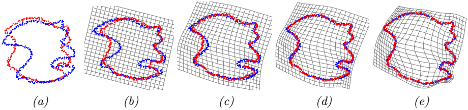
Fig. 5. Noisy case: registration results of a noisy 2D shape [20] using the proposed approach (SD-FFD); \lambda \in \{10^5, 10^3, 10^2, 1\} from (b) to (e) respectively
