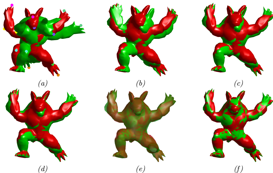
Fig. 7. 3D case: registration results of a deformed 3D shape [19] using the proposed approach (SD-FFD); (a) initial configuration with the corresponding feature points; (b) result in iteration 2 with ( \lambda = \mu = 10^3 ); (c) iteration 5 with ( \lambda = 10^2 ); (d) iteration 10 with ( \lambda = 10 ); (e) iteration 15 ( \mu = 10^2 ); (f) iteration 25 with ( \lambda = 1, \mu = 10 )
